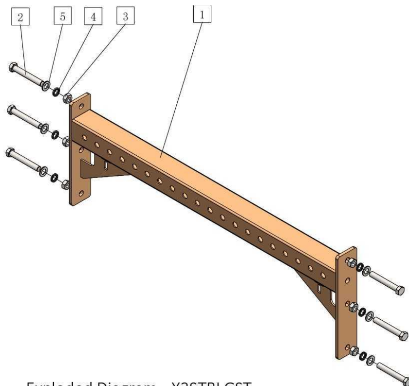
Exploded Diagram - X3STBLGST
