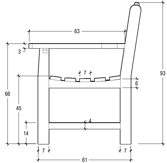
SIDE VIEW SCALE 1 : 15
