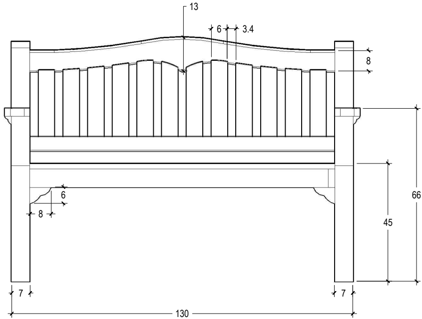
FRONT VIEW SCALE 1 : 15
