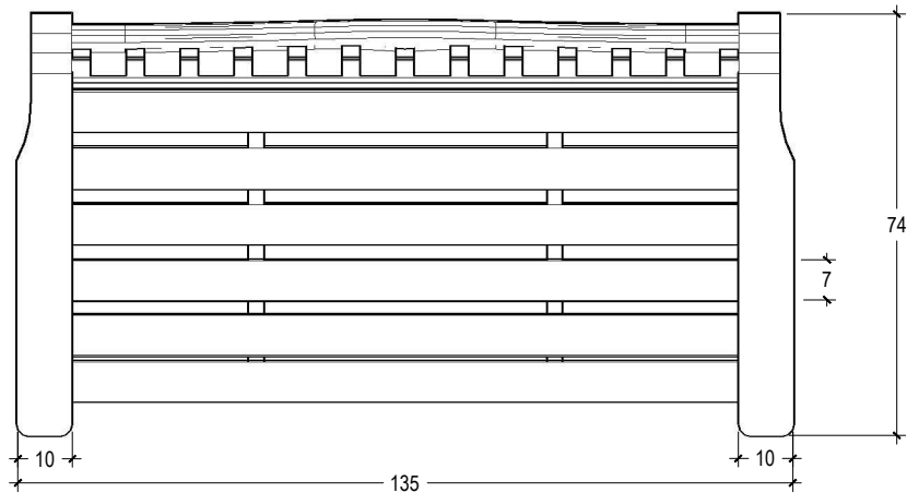
TOP VIEW SCALE 1 : 15
