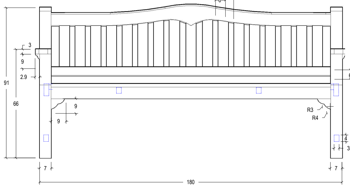
FRONT VIEW SCALE 1 : 14
